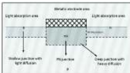
Selective Emitter cell
